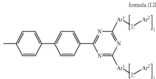
formula (I.IIc)
