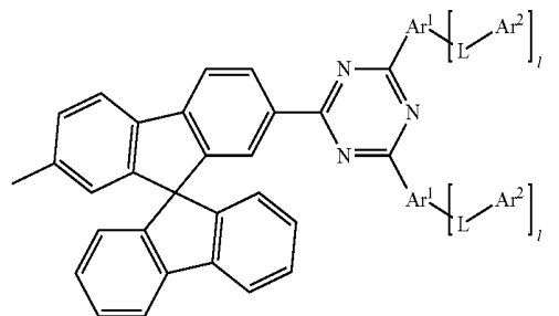
formula (I.IIe)
