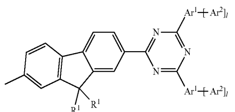
formula (I.IIi)
