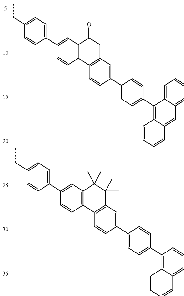
formula (VII)
