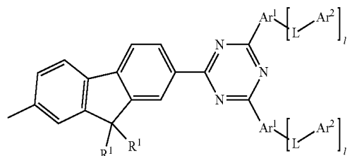
formula (I.IId)
