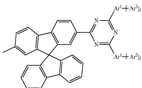
formula (I.IIj)
