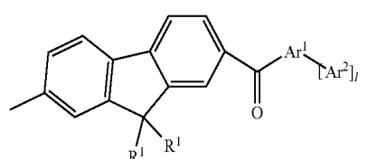
formula (I.Ih)
