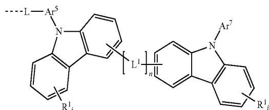
formula (IV)
