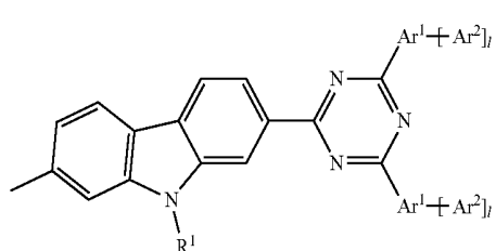
formula (I.IIj)
