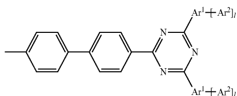
formula (I.IIh)
