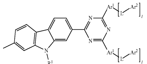
formula (I.IIe)
